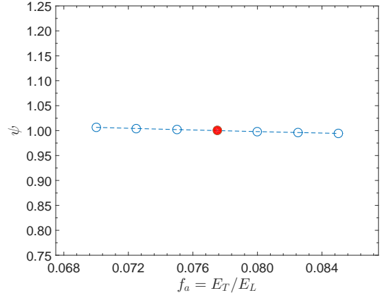
(d) Relative between \psi and E_T (with E_L = 13500 MPa, f_b = 0.0810 )
