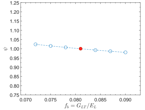
(f) Relative between \psi and G_{LT} (with E_L = 13500 MPa, f_a = 0.0775 )
